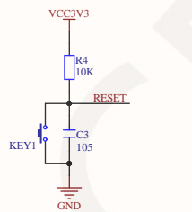
Key reset circuit
