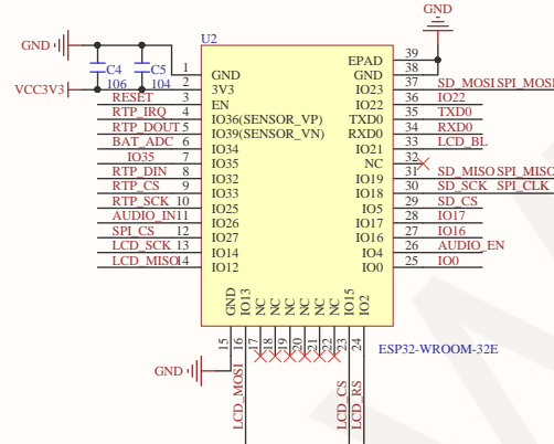
ESP32-WROOM-32E Main control circuit
