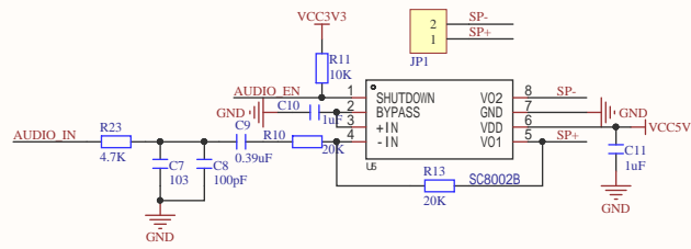
Audio power amplifier circuit
