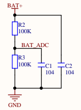
Battery level detection circuit
