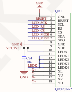
18P LCD panel wire welding interface
