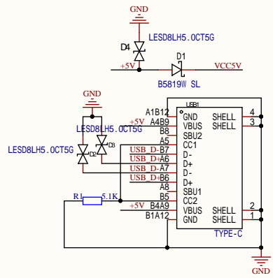
Type-C Interface circuit
